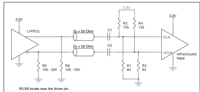
FIGURE 5. HiPerClockS CLK/nCLK INPUT DRIVEN BY 3.3V LVPECL DRIVER WITH AC COUPLE
